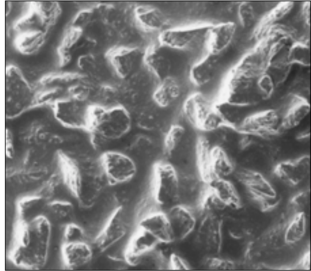
This surface profile of PLANARMET AL demonstrates the tight particle bond, 50x.
