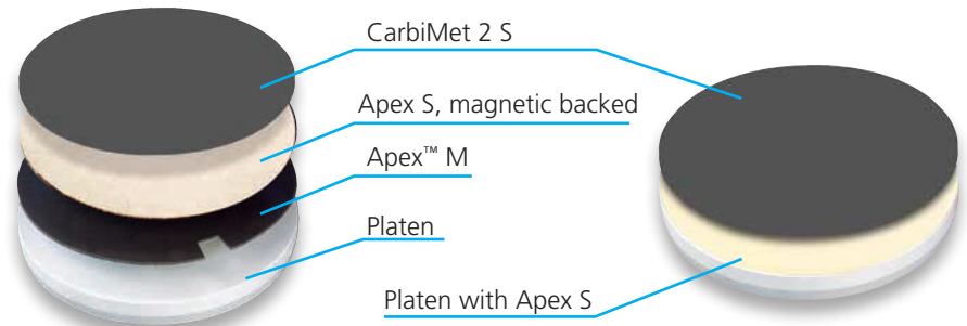
The Apex S Quick Change System can be used in different configurations as shown above.
